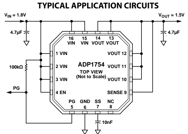
Figure 1. ADP1754 with Fixed Output Voltage, 1.5 V
